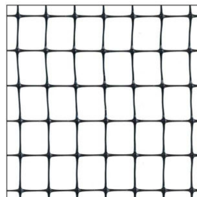
Bi-Oriented Net
